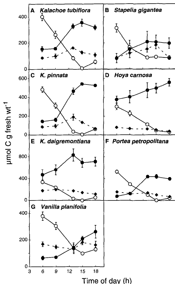
Figure 2. Concentration of malate (○), starch (●), and soluble sugars (Glc plus Fru plus Suc) (◆) in the CAM species K. tubiflora (A), S. gigantea (B), K. pinnata (C), H. carnosa (D), K. daigremontiana (E), P. petropolitana (F), and V. planifolia (G). Dawn was at approximately 5:50 AM and sunset at 6:10 PM. Values are the means \pm SE for six determinations. In some cases error bars are obscured by symbols.
