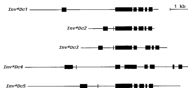
Figure 2. Structural maps of genomic clones for cell wall invertase and vacuolar invertase from carrot. Inv*Dc1 , Inv*Dc2 , and Inv*Dc3 code for cell wall invertase and related enzymes (Lorenz et al., 1995). Inv*Dc4 and Inv*Dc5 code for isoform I and II of vacuolar invertase (M. Hardegger and A. Sturm, unpublished results). The coding regions are represented as black boxes, with intervening and non-coding sequences shown as lines.
