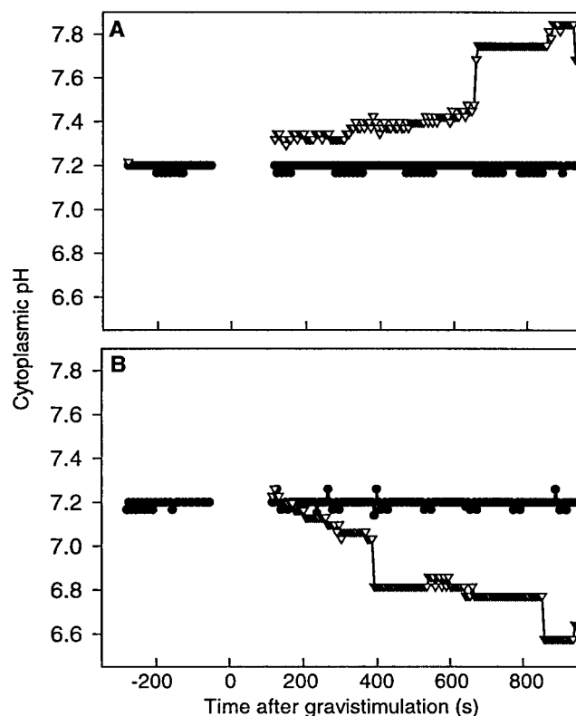
Figure 5. Statistically significant changes in pH c occur in columella cells of Arabidopsis following gravistimulation ( t = 0 s). A, Tier 2 cells ( n = 10 ) alkalinize immediately following gravistimulation. ●, Control; ▽, after gravistimulation. B, Tier 3 cells ( n = 10 ) acidify 180 s following gravistimulation. ●, Control; ▽, after gravistimulation.
