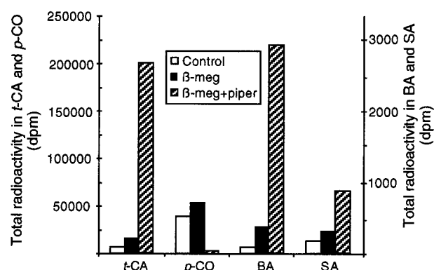
Figure 4. Effect of piperonylic acid on the distribution of total radioactivity (dpm) associated with total t -CA, p -CO, BA, and SA after feeding [ ^{14}\text{C} ] t -CA to elicited tobacco cells. BY-2 cells were elicited with 50 nM \beta -megaspermin for 12 h in presence (hatched bars) or in absence (black bars) of 10 \mu\text{M} piperonylic acid. Control cells (white bars) were treated with water. [ ^{14}\text{C} ] t -CA (2.2 \mu\text{mol} , 4.5 \text{mCi mmol}^{-1} ) was added during the last hour of elicitation. Total radioactivity associated with t -CA, p -CO, BA, and SA was determined after acid and base hydrolysis of the extracts. Note the difference of the scale used for t -CA and p -CO, and BA and SA. Piper, Piperonylic acid; \beta -meg, \beta -megaspermin. A duplicate experiment gave essentially the same results.
