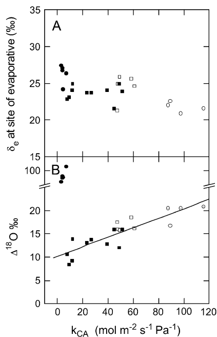
Figure 2. The isotopic composition (‰) of the water at the site of evaporation ( \delta_e ) and the oxygen isotope discrimination ( \Delta^{18}\text{O} ) as a function of the rate constant of leaf CA ( k_{\text{CA}} mol m -2 s -1 Pa -1 ). Values of \delta_e were calculated as described in the text using Equation 1 and source water ( \delta_s ) was -5.3 \pm 0.3 ‰. The line represents a linear regression ( R^2 = 0.87 ) for all data except the plants with high \Delta^{18}\text{O} values. Symbols and gas exchange conditions are as in Figure 1 and \delta values are expressed in reference to VSMOW.
