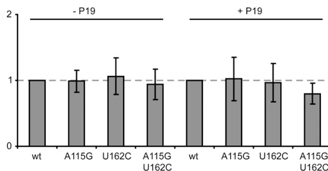
Figure 3. Analysis of RNA accumulation from the wild-type (wt) and mutant 5' leader sequences either in the absence or presence of P19. Values indicate the average proportion of transcripts relative to the wild-type leader from three extracts \pm SE.
