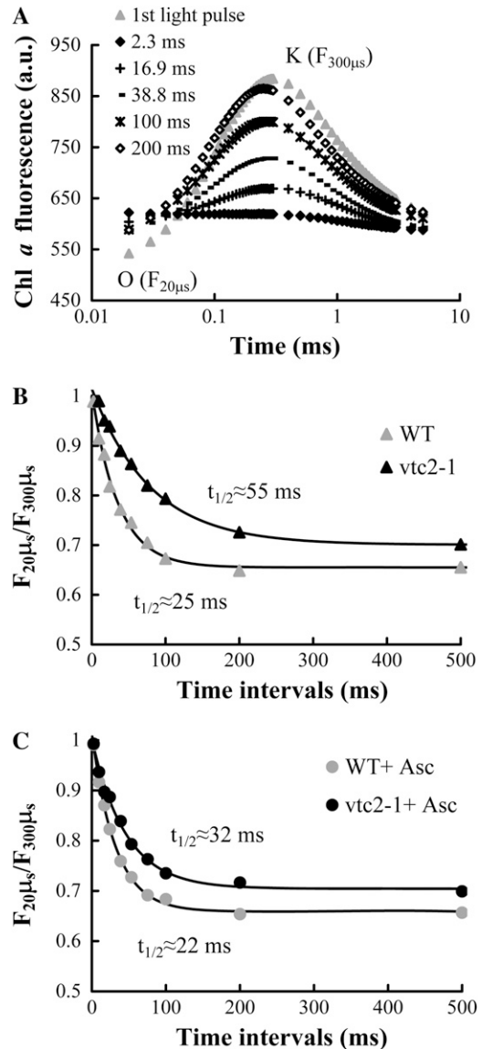
Figure 2. Dependence of the recovery of the K peak of the fast Chl a fluorescence transient in heat-treated wild-type and Asc-deficient Arabidopsis plants ( vtc2-1 mutant) on the dark interval between the light pulses. A, Fast Chl a fluorescence transients measured on heat-treated (49°C, 40 s) wild-type (WT) leaves during 5-ms light pulses that were spaced 2.3 to 200 ms apart, as indicated. The fluorescence curves are averages of eight to 10 measurements. a.u., Arbitrary units. B and C, Regeneration of the K peak (calculated as F_{20\mu\text{s}}/F_{300\mu\text{s}} ) as a function of dark intervals between the light pulses in heat-treated wild-type and vtc2-1 plants in the absence (B) and the presence (C) of externally supplied Asc (incubation of leaves in 20 mM Asc for 2 h in low light). The points are mean values from four to eight individual measurements that were fitted with exponentials for the determination of the half-recovery time. The error of the fitting was 5% to 6%.
