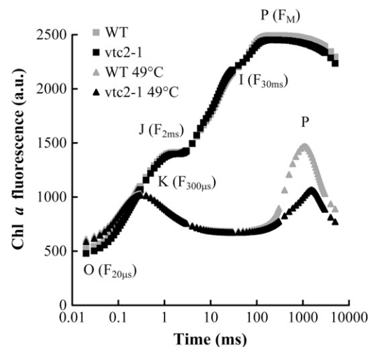
Figure 1. Fast Chl a fluorescence transients (OJIP curves) of untreated and heat-treated (49°C, 40 s) wild-type (WT) and Asc-deficient vtc2-1 Arabidopsis thaliana mutant plants measured at 3,500 \mu\text{mol m}^{-2} \text{s}^{-1} photon flux density. The approximate positions of the different steps of the OJIP transient and of the K peak are indicated in parentheses. The curves are averages of eight to 10 measurements. The excitation light was produced by three 650-nm LEDs, and the Chl a fluorescence was measured at wavelengths above 700 nm. a.u., Arbitrary units.
