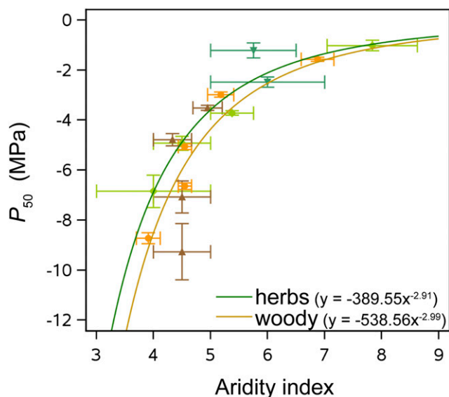
Figure 2. P_{50} versus aridity index in herbs and woody species. Herbaceous and woody species that are more resistant to embolism formation (more negative P_{50} ) grow in drier environments (lower aridity index; Julve, 1998). P_{50} values were averaged for each plant group every 2 MPa (light-green diamonds, grasses; dark-green triangles, herbaceous eudicots; orange circles, woody angiosperms; brown triangles, woody gymnosperms). Error bars show SE.
