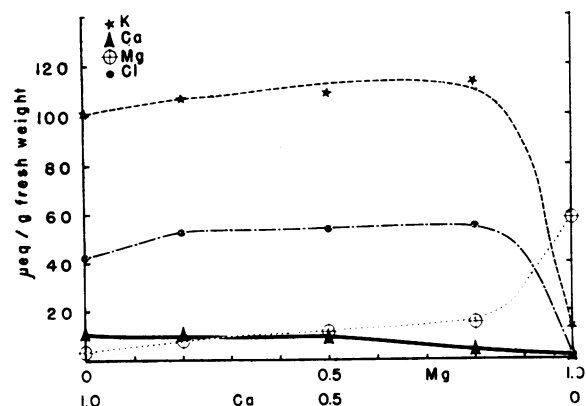
FIG. 6. Influence of Ca/Mg on the Mg, K, Ca, and Cl contents of excised soybean roots after 24 hr in 1 mM KCl and 5 mM (Ca + Mg)Cl 2 solutions. (Note the change in ordinate scale after Fig. 5.)
