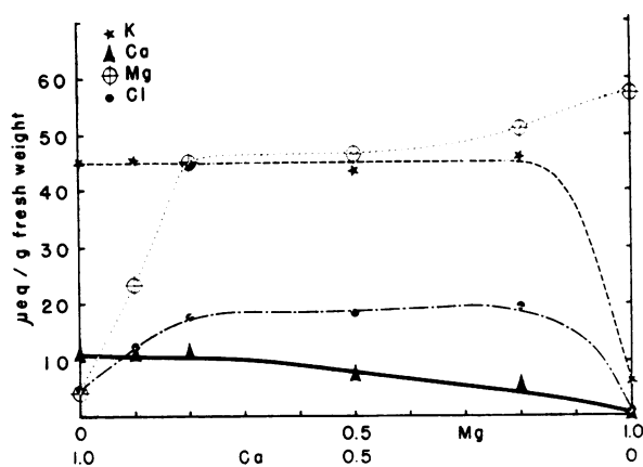
FIG. 5. Influence of Ca/Mg on the Mg, K, Ca, and Cl contents of excised soybean roots in 5 mM (Ca + Mg)Cl 2 solutions for 24 hr.
