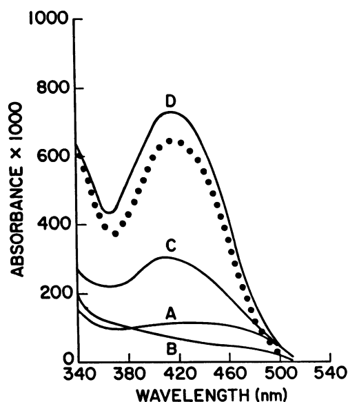
Figure 1. Data from typical experiment with duckweed ( Lemna minor ), in which hydroxyl radicals were trapped and measured as methane sulfonic acid. Visible absorbance spectra of colorimetric assay of untreated leaves (A), DMSO-only-treated leaves (B), paraquat-only-treated leaves (C), and paraquat + DMSO-treated leaves (D). Dotted line represents 300 nmol MSA standard.
