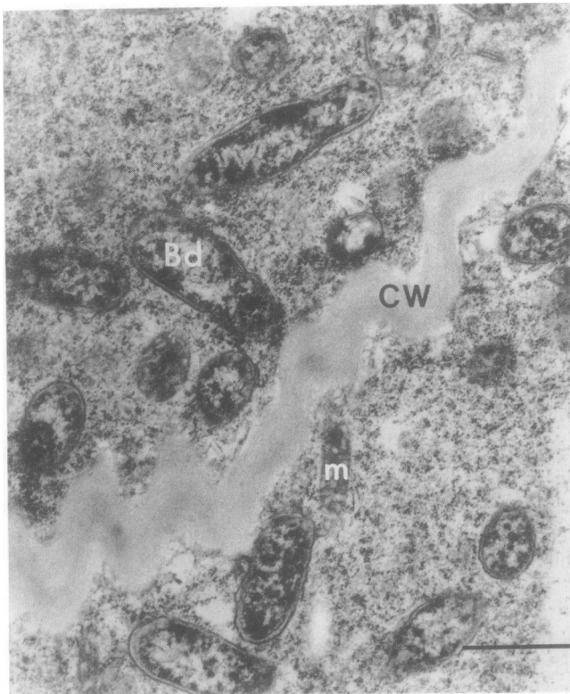
Figure 2. Electron micrograph ( \times 19,000 ) of the symbiotic zone of a 2-1/2 week-old Fix^- nodule induced by Rm1021- \alpha MT8 (courtesy of Ann Hirsch and Carol Smith). Bar = 1 \mu m. Bd, bacteroid, CW, cell wall; m, mitochondrion.
