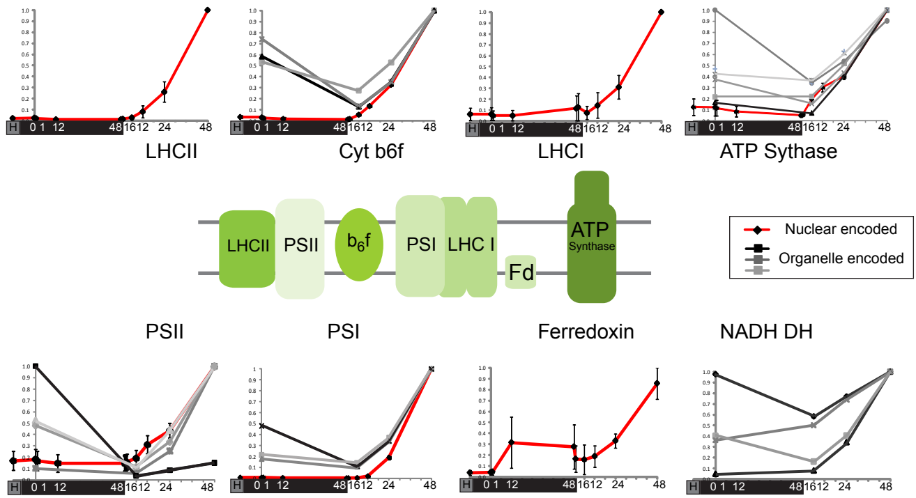
Supplementary Figure 4. Coordination of nuclear and organelle encoded components of the chloroplast photosynthetic ETC. Expression values derived from microarray analysis of nuclear encoded components of the chloroplast were profiled in parallel to corresponding components encoded by the chloroplast genome by qRT-PCR. The microarray data spanned ten time points, while the qRT-PCR included only four time points.
